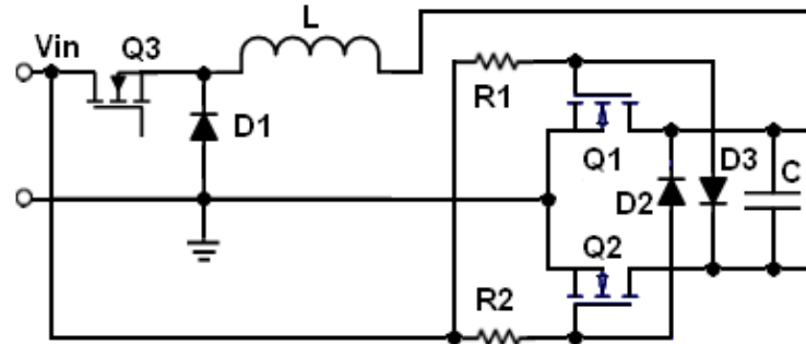
Gambar 4. Topologi pushpull inverter
