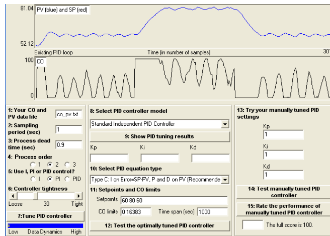
Gambar 2. Standard Independent PID Controller
