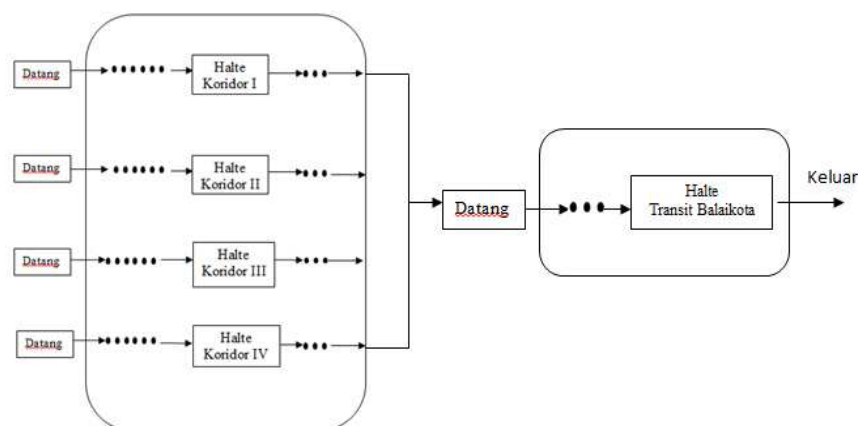
Gambar 2. Sistem Antrian Halte Operasional BRT Semarang
