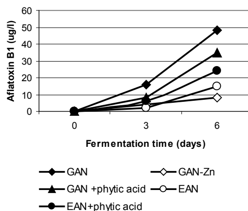
Figure 3 Production of aflatoxin B1 during the growth of mold
