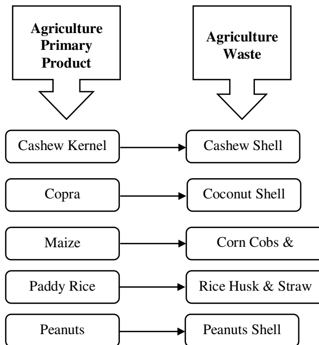
Figure 2. Agriculture product and their waste
