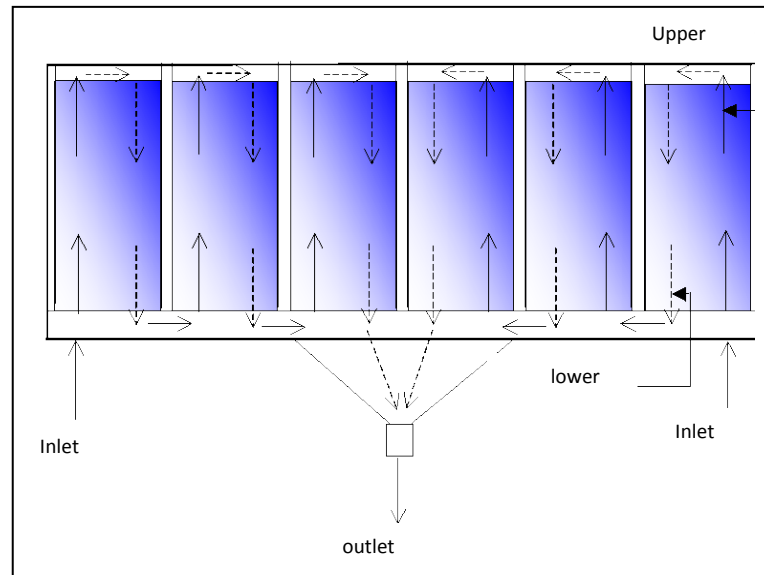
Fig. 6. The collector array for the solar drying system
