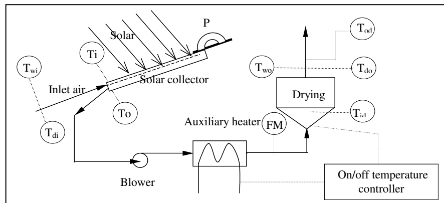
Fig. 7. Schematic of the solar assisted drying system
