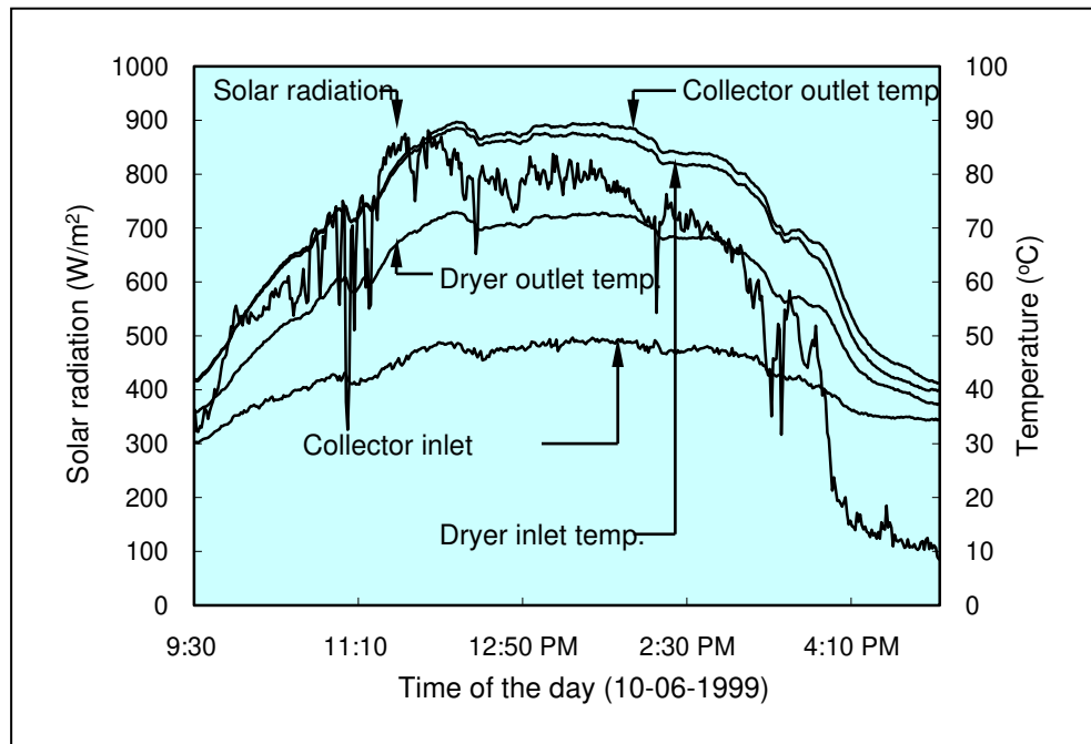
Fig. 8 Variations of the solar radiation and various temperatures (dryer inlet and outlet, collector inlet and outlet)
