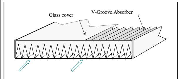
Fig. 2. Configuration of the V-groove
