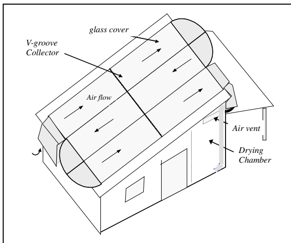
Fig. 1. Configuration of the V-groove solar drying system
