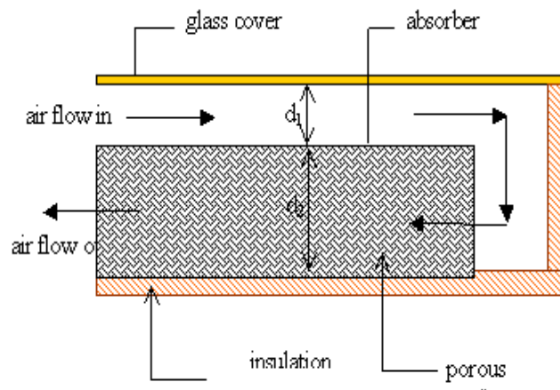
Fig. 5. The schematic of a double-pass solar collector with porous media in the second channel. ( d_1 = 3.5 cm, d_2 = 10.5 cm).
