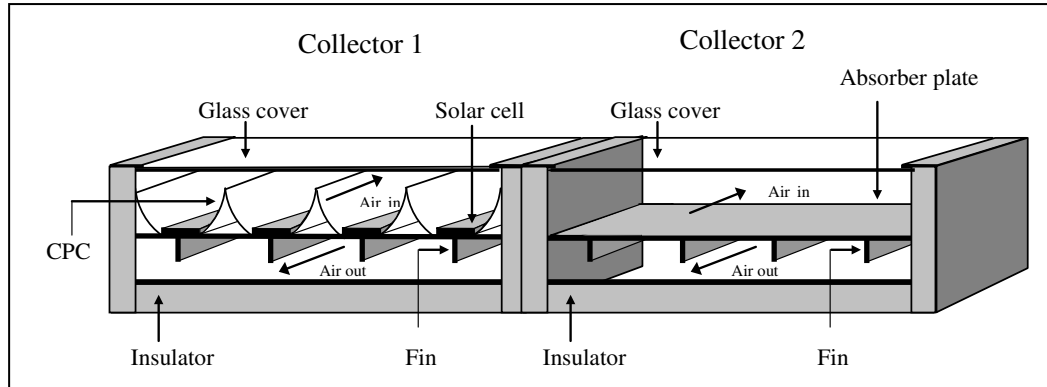
Fig. 10. The schematic diagram of photovoltaic- thermal solar collector
