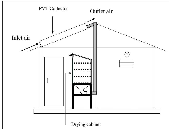
Fig. 12. Side view of PVT solar drying system
