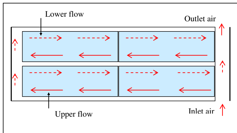
Fig. 11. The collector array for the solar drying system.
