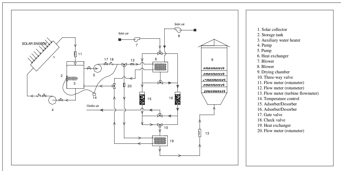
Fig. 9 The schematic of the solar assisted dehumidification drying system.
