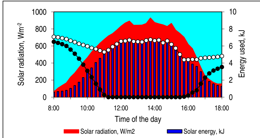
Fig. 3. The contribution of the auxiliary and solarenergy to maintain the drying chamber temperature of 50°C for the drying of herbal tea.
