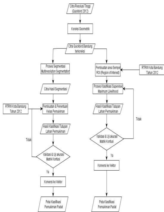
Diagram II.1. Tahapan analisis
