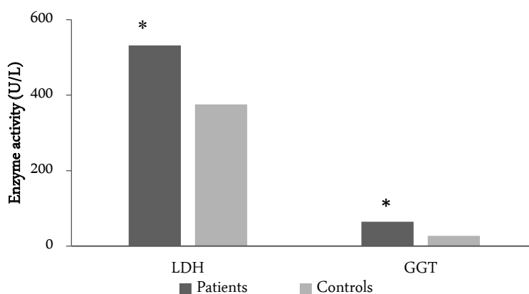
Figure 1. Overall comparison of LDH and GGT in BC patients and controls
