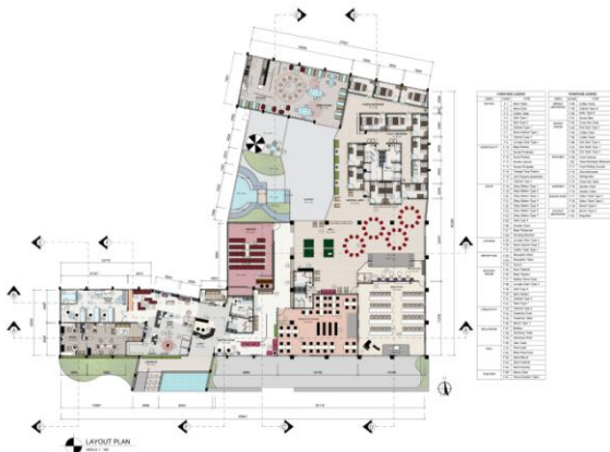
Gambar. 4. Layout EDCC
