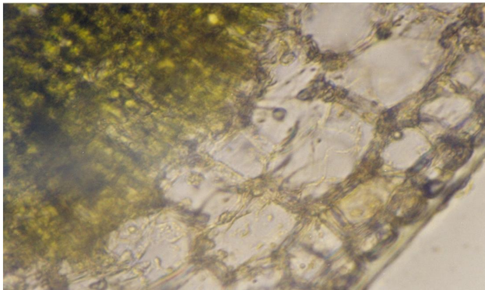
Fig. 9. At riverine end with lower salinity less thickness of water storage tissue. --- Palisade layer more in thickness.
