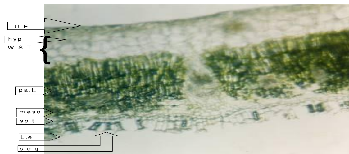
Fig. 4. A typical transverse section of leaf of Avicennia marina showing upper epidermis (U.E.), Hypodermis (hyp), Mesophyll (meso), lower epidermis (L.e). Hypodermis- water storage tissue (W.S.T.) - Mesophyll—palisade (pa.t.), spongy tissue (sp.t.) - spongy tissue more with reduced salinity - lower epidermis—salt extruding glands. (s.e.g.)
