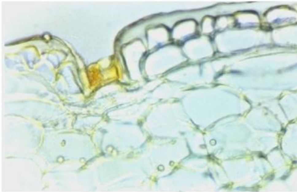
Photo plate 5: Upper epidermis covered with a thick cuticle. It has salt accumulating gland at intervals.
