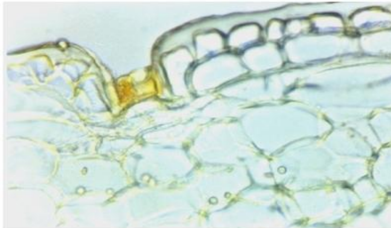
Fig. 5. Upper epidermis covered with a thick cuticle. It has salt accumulating gland at intervals.
