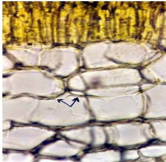
Fig. 8. At seaward end with higher salinity water storage tissue is more in thickness.
