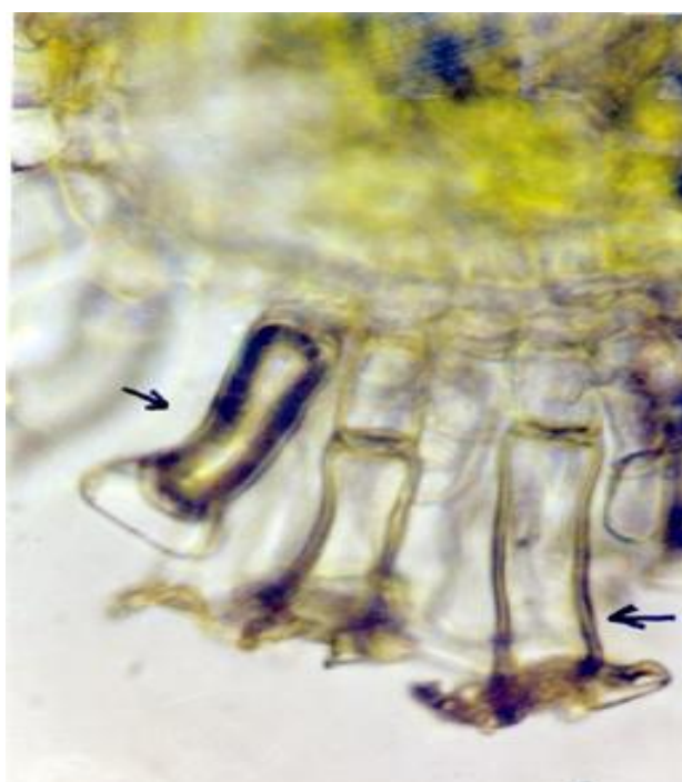
Fig. 7. At higher salinity salt extruding glands are taller and slender
