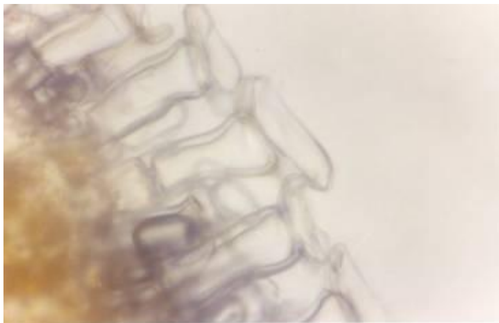
Photoplate 6: At lower salinity salt extruding glands are shorter and broader.
