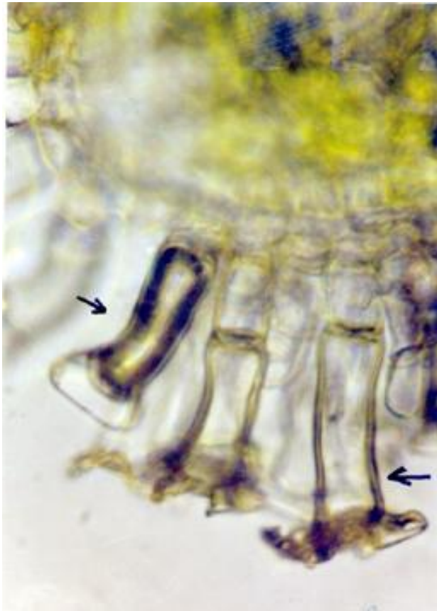
Photo plate 7: At higher salinity salt extruding glands are taller and slender.
