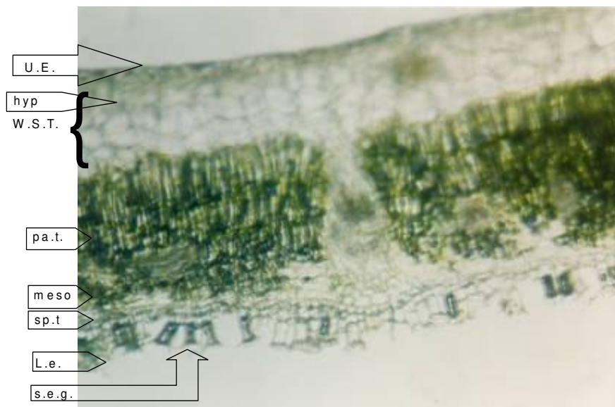
Photo plate 4: A typical transverse section of leaf of Avicennia marina showing upper epidermis (U.E.), Hypodermis (hyp), Mesophyll (meso), lower epidermis (L.e). Hypodermis- water storage tissue (W.S.T.)
