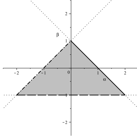
FIGURE 3. In this Figure, we have plotted the area in the (\alpha, \beta) -plane where the sequence (1) converges to zero. This is done by analyzing the magnitude of \lambda_1 and \lambda_2 .
