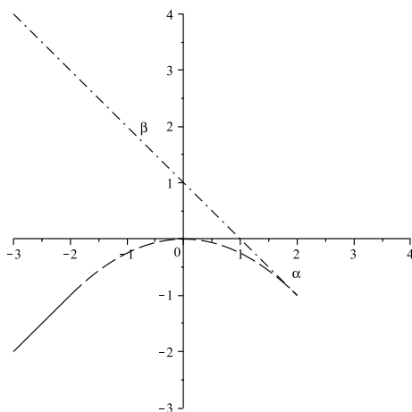
FIGURE 1. In this Figure, we have plotted the area in the (\alpha, \beta) -plane where |\lambda_1| < 1 . The domain is bounded by the line \alpha + \beta = 1 which is plotted using a dashed and dotted line, the parabola: \alpha^2 + 4\beta = 0 which is plotted using a dashed line, and \beta - \alpha = 1 which is plotted using a solid line.
