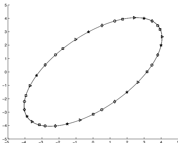
FIGURE 4. In this figure we have plotted an ellipse which is formed by 5000 iterations of (1) for \alpha = 1.25 and \beta = -1 . The initial conditions are x_1 = 4 and x_2 = 3 . This iterations densely fill up an ellipse. The horizontal axis is x_n while the vertical axis is x_{n+1} . On the ellipse, there are five 7-periodic sequences (see Definition 2.1) which are obtained by 150 iterations of (1) for \alpha = 2 \cos \frac{2\pi}{7} and \beta = -1 , but five different sets of initial conditions: \{x_1 = 3.4589, x_2 = 0.5159\} ( \circ ), \{x_1 = -2.2150, x_2 = -4.0321\} ( \diamond ), \{x_1 = -3.3212, x_2 = -0.2652\} ( \star ), \{x_1 = 2.4215, x_2 = 4.0486\} ( \triangleright ), and \{x_1 = 3.1707, x_2 = 3.1707\} ( \square ).
