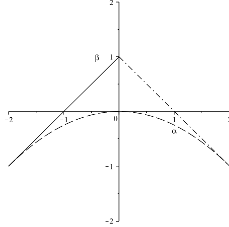
FIGURE 2. In this Figure, we have plotted the area in the (\alpha, \beta) -plane where |\lambda_1| < 1 and |\lambda_2| < 1 . The domain is bounded by the line \alpha + \beta = 1 which is plotted using a dashed and dotted line, the parabola: \alpha^2 + 4\beta = 0 which is plotted using a dashed line, and \beta - \alpha = 1 which is plotted using a solid line.
