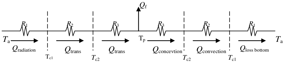
Figure 6 Thermal resistance of ETSC.
