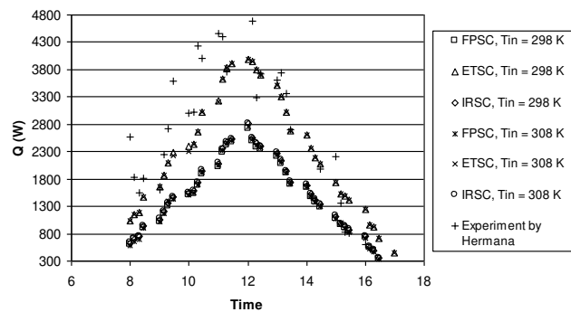
(b) Characteristics of absorbed heat by working fluid at different inlet temperature of working fluid.
