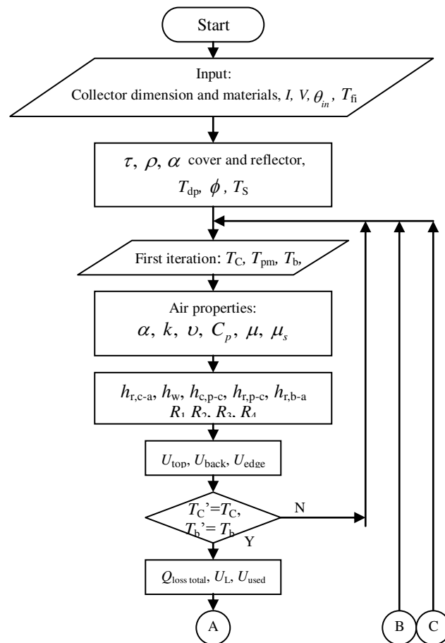
Figure 8 Flow chart of numerical calculation of solar collectors.
