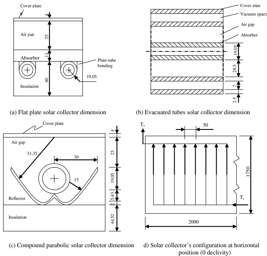
Figure 2 Schematic dimension and configuration of solar collectors (unit in mm).
