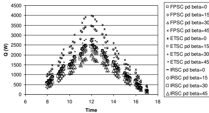
(a) Characteristics of absorbed heat by collector
