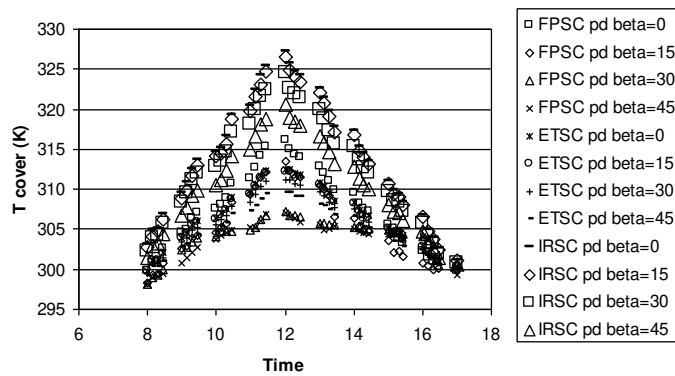
(e) Characteristics of cover plate temperature.
