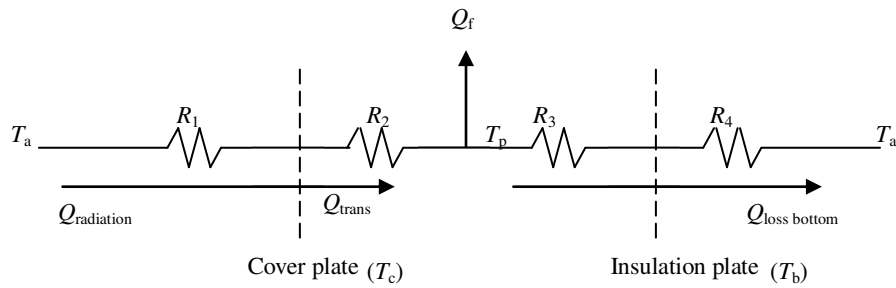
Figure 5 Thermal resistance of FPSC.
