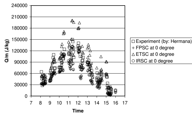
(a) Characteristics of absorbed heat by working fluid at 0 inclination of solar collector.
