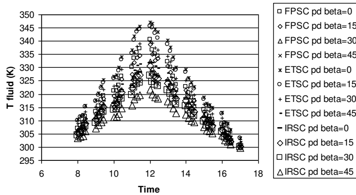
(d) Characteristics of outlet temperature of working fluid
