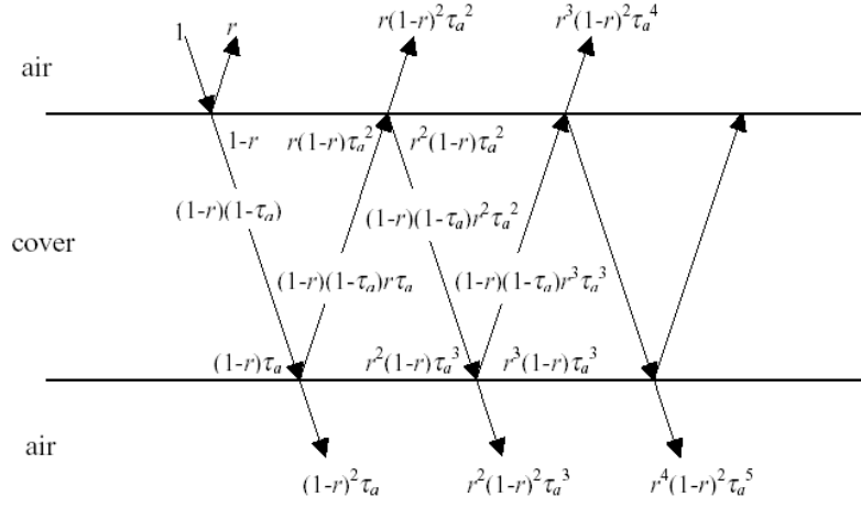
Figure 3 Ray tracing techniques for obtain transmissivity, reflectivity and absorptivity of single cover plate [7].
