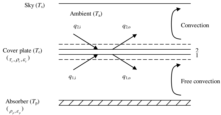
Figure 4 Heat transfer at single cover plate.
