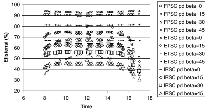
(c) Characteristics of efficiency
