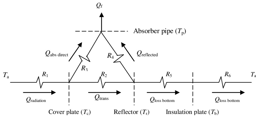
Figure 7 Thermal resistance of CPSC.
