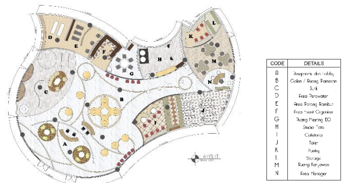
Gambar 1. Layout
