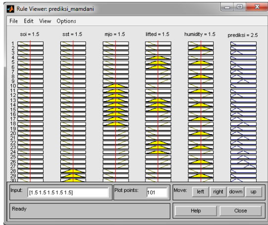
Gambar 10. Rule Viewer tipe Mamdani
