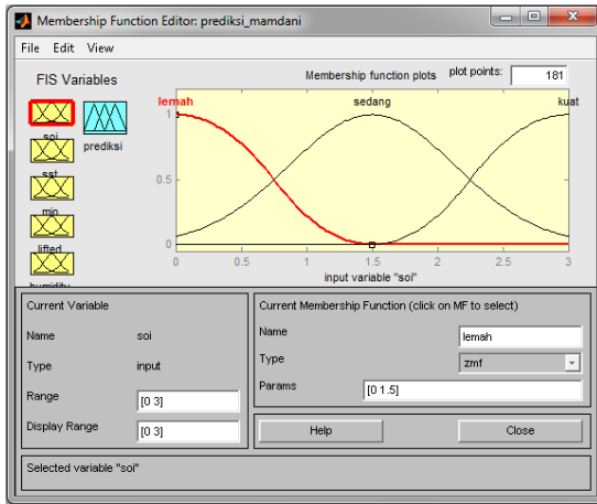
Gambar 7. Membership Function input
