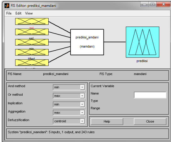
Gambar 6. FIS Editor tipe Mamdani
