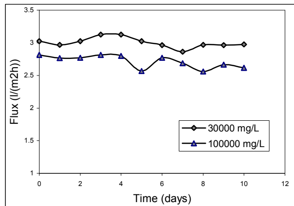
Fig. 9. The flux stability on operation time at Tf/Tp = 80/25°C and feed velocity 0.2 m/s
