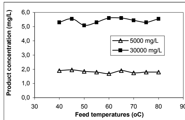
Fig. 8. The effect of feed temperature on product quality at permeate temperature of 25°C and feed velocity of 0.05 m/s
