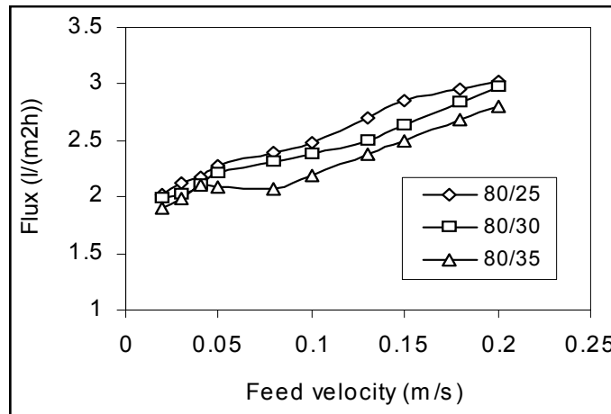
Fig. 5. The effect of feed velocity on flux at various Tf/Tp with feed concentration of 30000 mg/L
