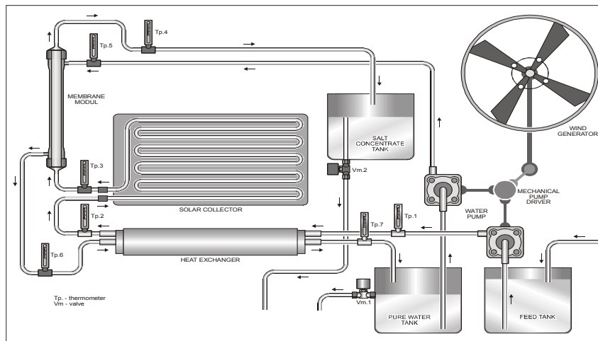
Fig. 3. Schematic representation of LLMC powered by solar and wind energy
