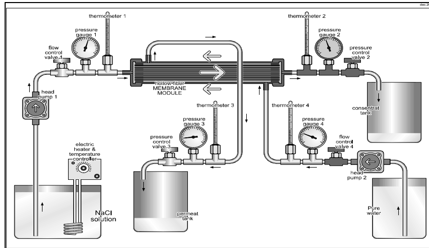
Fig. 2. Schematic representation of experimental apparatus
