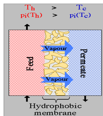
Fig. 1. Schematic representation of LLMC
