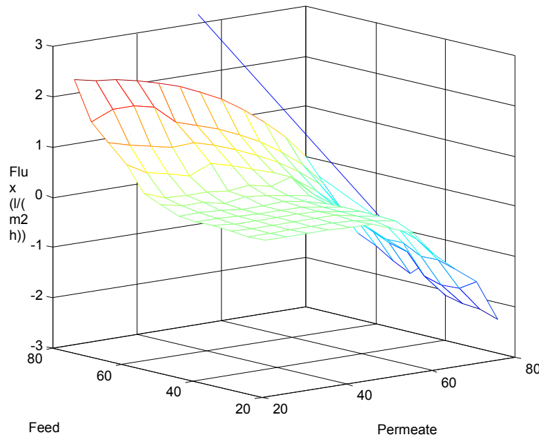
Fig. 4. The flux profile functions of the feed and permeate temperature at v = 0.05 m/s and NaCl = 30000 mg/L
