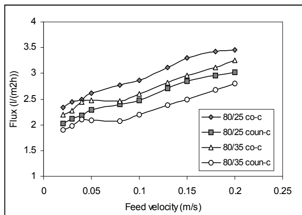
Fig. 7. Flux comparison between co-current and counter current modes at feed concentration of 30000 mg/L
