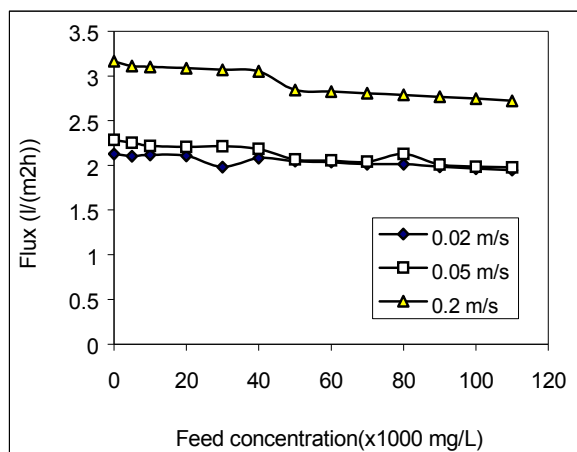
Fig. 6. The effect of feed concentration on flux at various feed velocities and T_f/T_p = 80/30^\circ\text{C}
