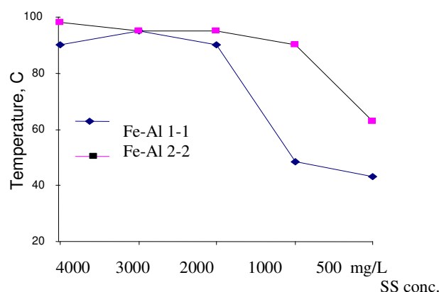
Fig. 2 Influence of initial SS concentration on final temperature
