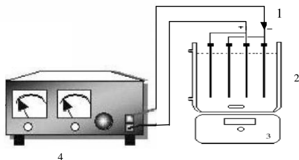
Fig. 1 The electro-coagulation experimental apparatus (1). Electrode; (2). Electro-coagulator; (3). Magnetic stirrer; (4). Power supply
