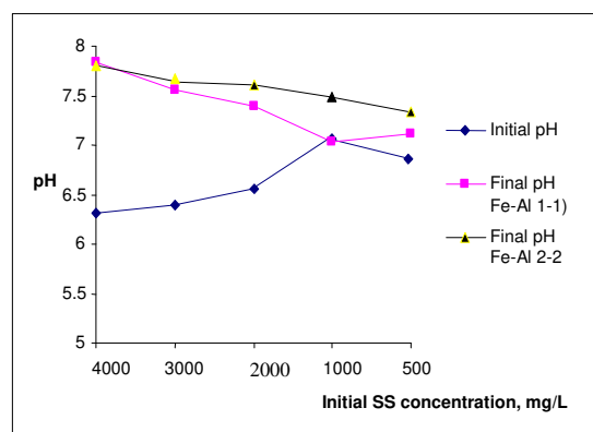
Fig. 4 The effect of initial pH of wastewater to final pH
