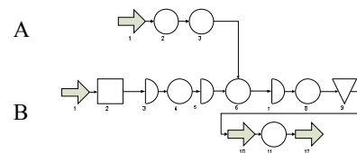
Gambar 3. Peta Aliran Proses Bay 2.1
