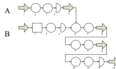
Gambar 3. Peta Aliran Proses Bay 2.1
