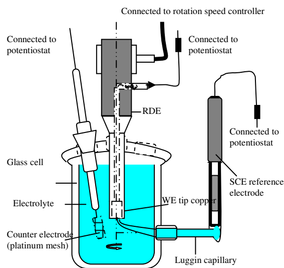
Figure 1 Diagram of three-electrode cell for electrochemical investigation
