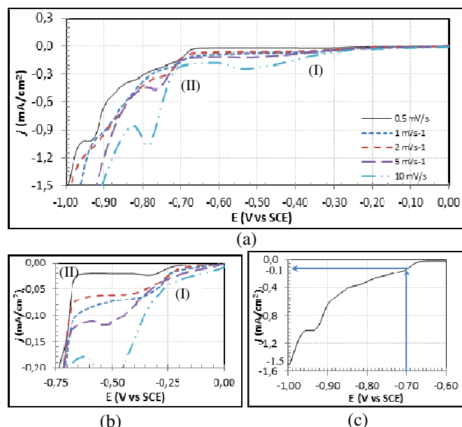
Figure 2 (a) Cathodic Polarisation Curves for 0.19 M nickel sulfamate at various scan rates, the RDE rotation speed was 0 rpm on copper substrate, (b) zoom of the low current density region to show the steady state condition (c) zoom of nickel deposition region for 0.5 \text{mVs}^{-1} scan rate.
