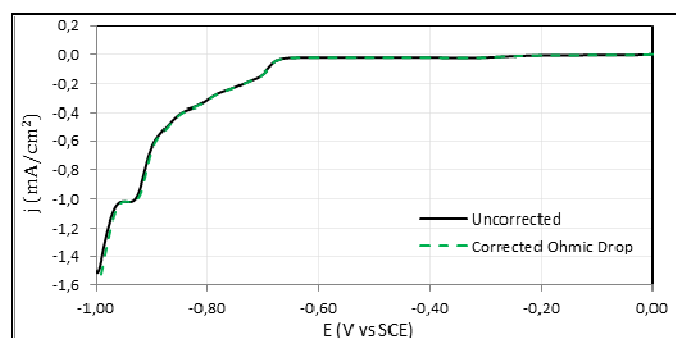
Figure 3. Comparison between cathodic polarisation Curves for 0.19 M nickel sulfamate with and without ohmic drop correction on copper substrate at 0.5 mV/s scan rate and 0 rpm RDE rotation speed.
