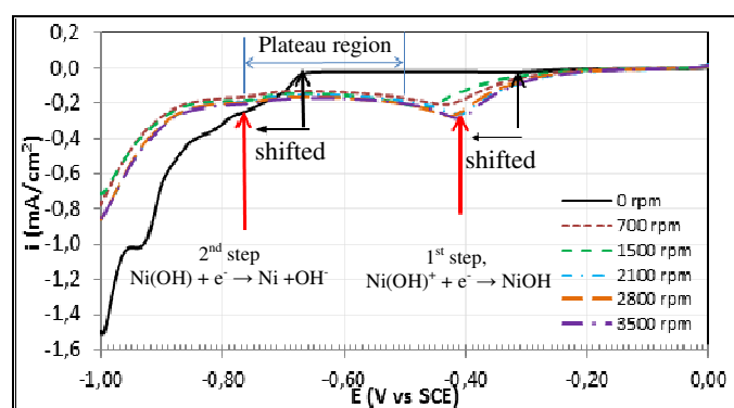
Figure 4. Cathodic Polarisation Curves for 0.19 M nickel sulfamate on copper substrate at 0.5 mV/s scan rate, the RDE rotation speed varied between 0 and 3500 rpm.
