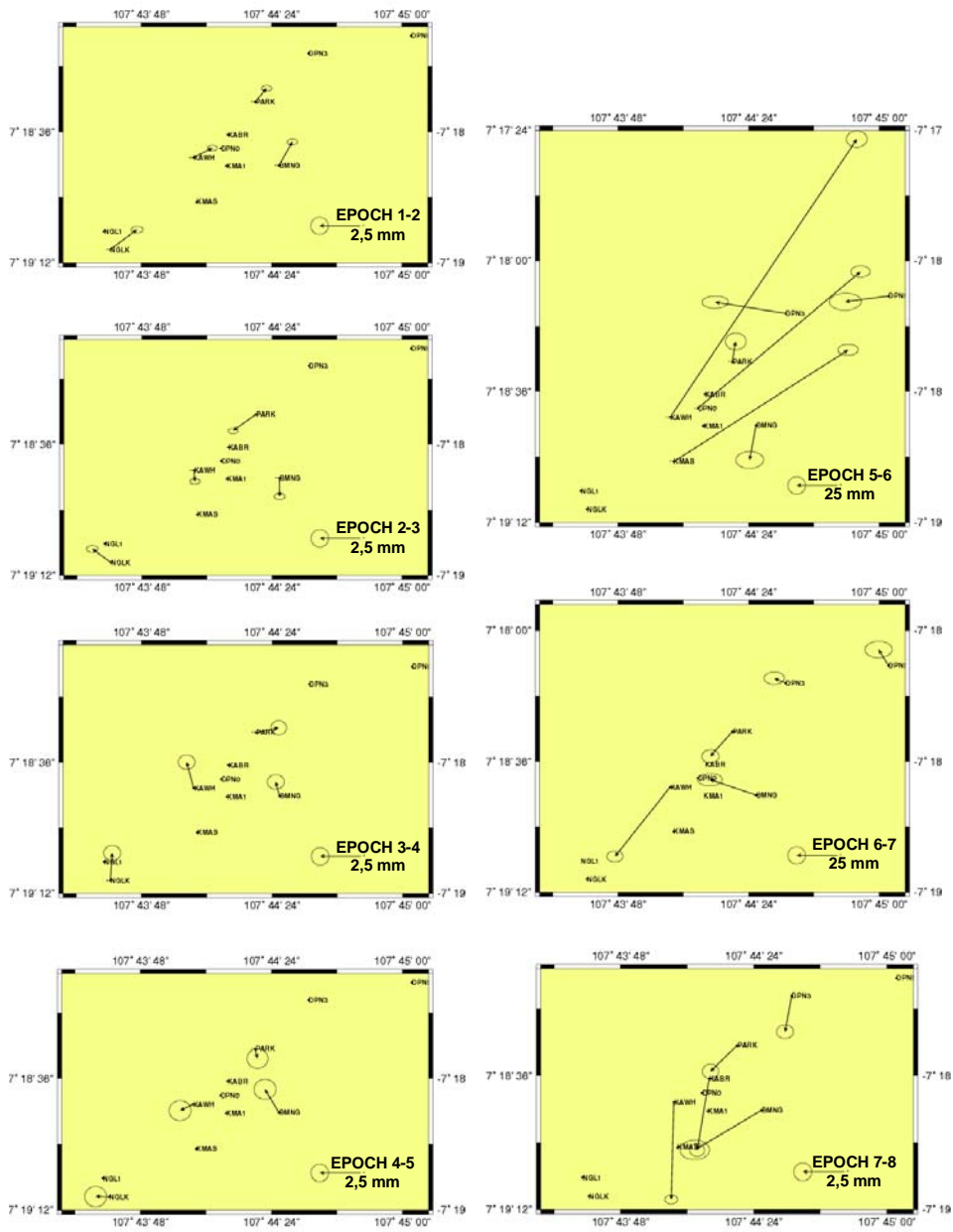
Figure 7 Vector displacement in horizontal direction.
