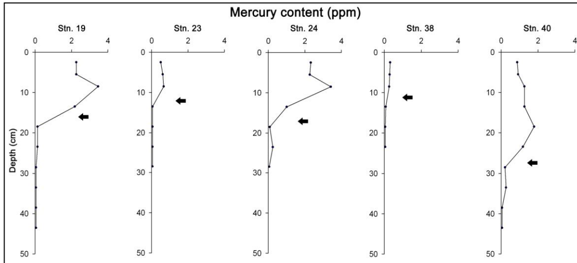
Fig. 5 Vertical distribution of mercury contents in core samples (arrow: first appearance of high mercury contents)
