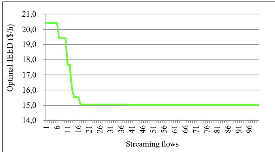
Figure 3 Convergence speed.
