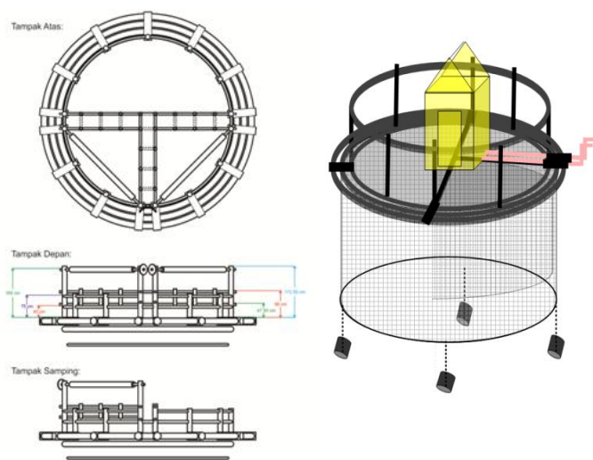
Figure 5. Design of floating rounded net - cage SDNRC-IMTA (patent application No : S00207106486 2014 ).
