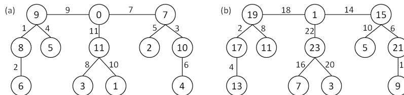
FIGURE 1. Graceful and simply sequential labelings of T_1 .
