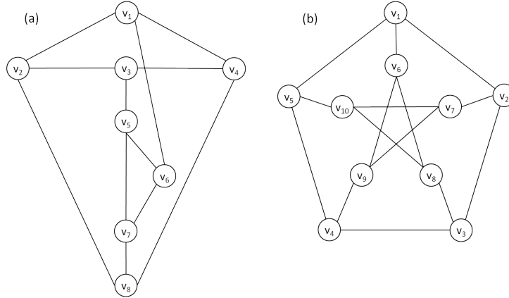
FIGURE 2. 3-Regular graph G1 and Petersen graph P
