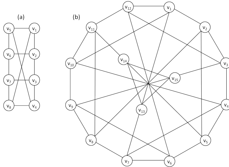
FIGURE 3. Mobius ladder G_2 and graph G_3
