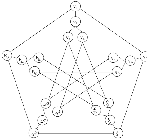
FIGURE 5. 3-Regular graph G_5 of order 20 and diameter 3
