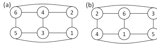
FIGURE 6. Labelings of G_6 showing NS(G_6) = 11 , NS^-(G_6) = 10 , NS^{sp}(G_6) = 1 , NS[G_6] = 16 , NS^-[G_6] = 12 , NS^{sp}[G_6] = 4
