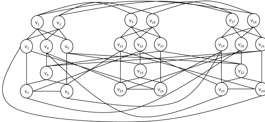
FIGURE 4. 5-Regular graph G_4 of order 24 and diameter 2
