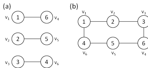
FIGURE 8. Graph G_7 and C_6 labeled to show a \{0, 3\} and \{1, 2\} -vertex magic labeling of C_6
