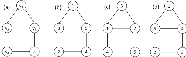
FIGURE 1. Minimax and maximin labelings of House graph H
