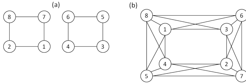
FIGURE 7. \Sigma labeling of the union of 2 C_4 's, and \Sigma' labeling of its complement
