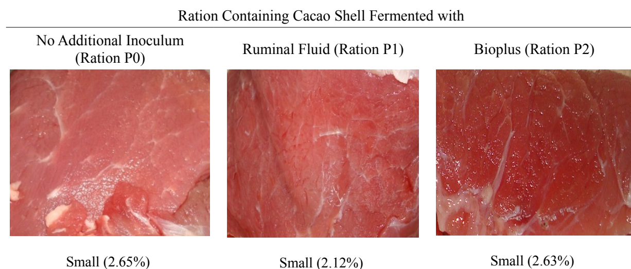
Figure 1. Marbling Evaluated at Rib Eye Area of Male Bali Cattle Fed Ration Containing Fermented Cacao Shell
