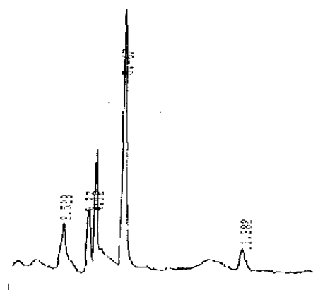
Fig. 3b. Chromatogram of STX standard (10 ng/ml)
