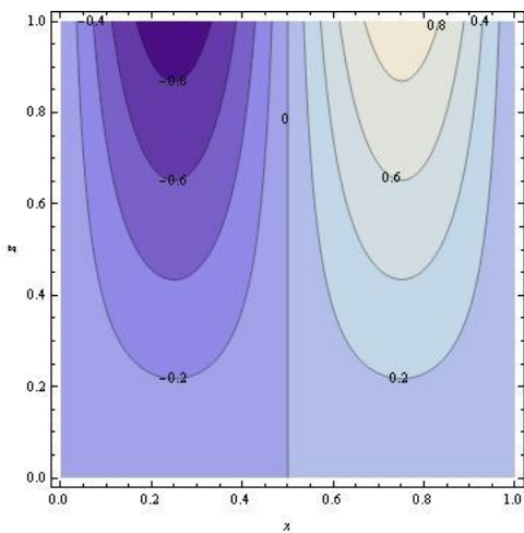
Fig. 3: Contour plot of first approximate solution U_1 at v = 1, y = 0.5 and t = 0.001 in xz -plane.
