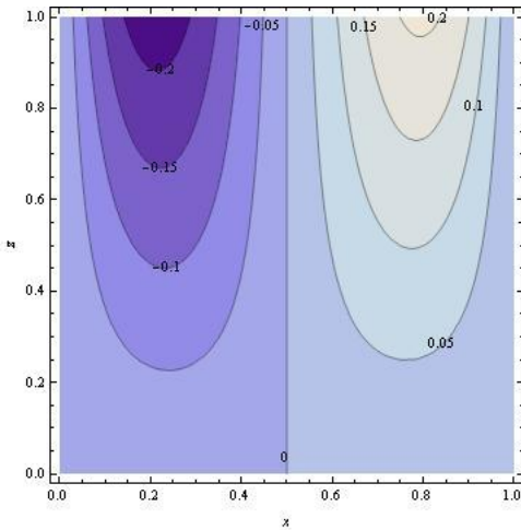
Fig. 7: Contour plot of first approximate solution U_1 at v = 1, y = 0.5 and t = 0.01 in xz -plane.
