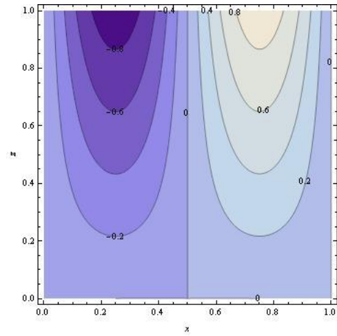
Fig. 4: Contour plot of second approximate solution U_2 at v = 1, y = 0.5 and t = 0.001 in xz -plane.
