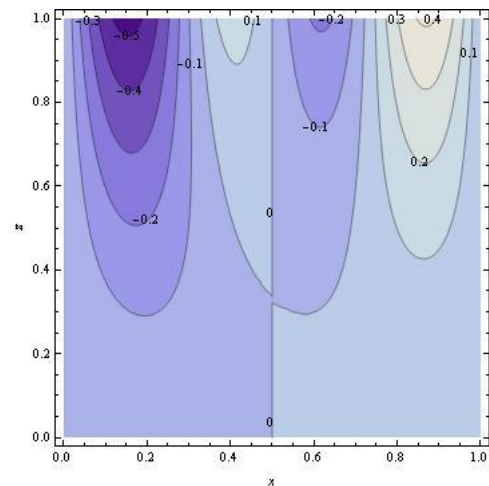
Fig. 11: Contour plot of first approximate solution U_1 at v = 0.1, y = 0.5 and t = 0.1 in xz -plane.
