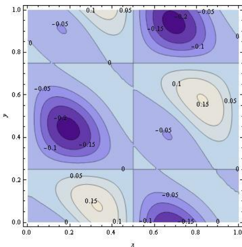
Fig. 9: Contour plot of first approximate solution U_1 at v = 0.1, z = 0.5 and t = 0.1 in xy -plane.
