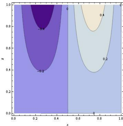
Fig. 8: Contour plot of second approximate solution U_2 at v = 1, y = 0.5 and t = 0.01 in xz -plane.
