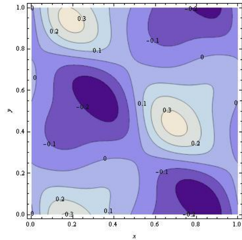
Fig. 10: Contour plot of second approximate solution U_2 at v = 0.1, z = 0.5 and t = 0.1 in xy -plane.
