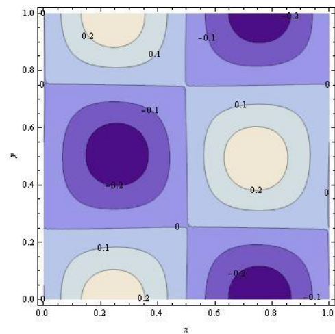
Fig. 6: Contour plot of second approximate solution U_2 at v = 1, z = 0.5 and t = 0.01 in xy -plane.
