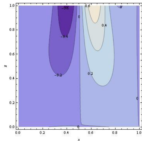
Fig. 12: Contour plot of second approximate solution U_2 at v = 0.1, y = 0.5 and t = 0.1 in xz -plane.
