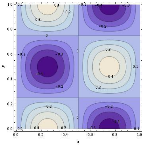
Fig. 1: Contour plot of first approximate solution U_1 at v = 1, z = 0.5 and t = 0.001 in xy -plane.
