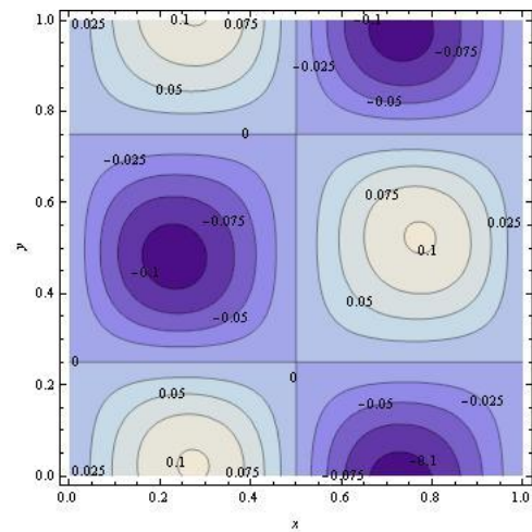
Fig. 5: Contour plot of first approximate solution U_1 at v = 1, z = 0.5 and t = 0.01 in xy -plane.
