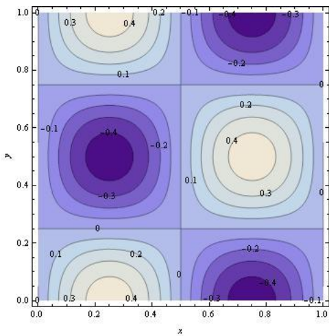
Fig. 2: Contour plot of second approximate solution U_2 at v = 1, z = 0.5 and t = 0.001 in xy -plane.
