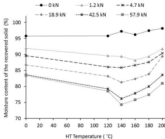
Fig.4 Effect of HT temperature and dewatering force on the moisture content of sludge cake
