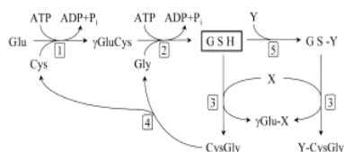
Figure 1. Mechanism of glutathione biosynthesis
