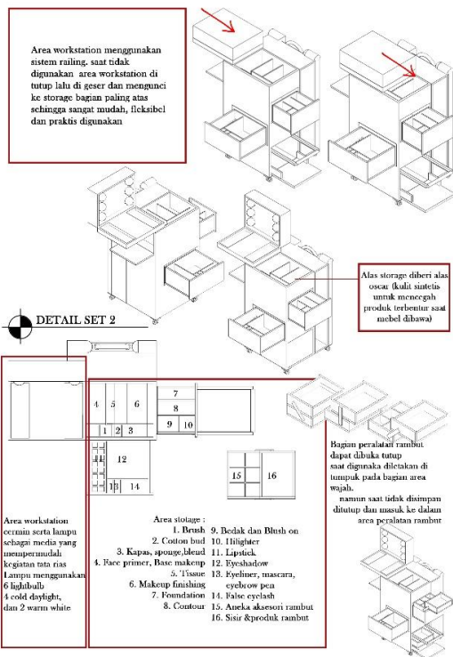
Gambar 18. Detail Mebel 2
