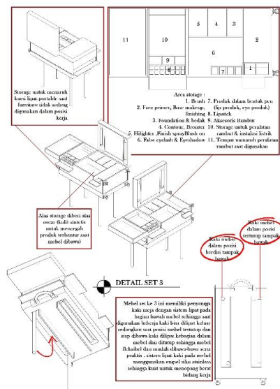
Gambar 21. Detail Mebel set 3
