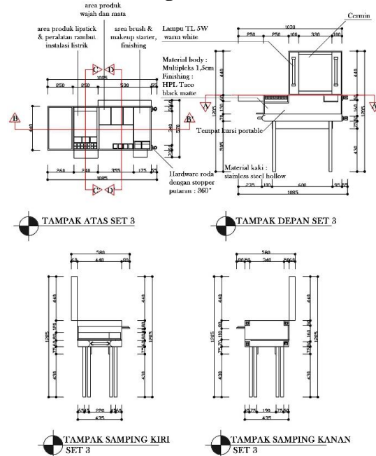
Gambar 20. Tampak Mebel set 3
