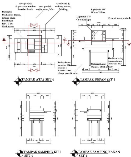
Gambar 23. Tampak Mebel set 4
