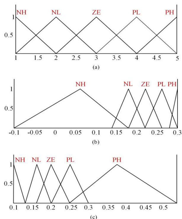
Figure 5 Membership functions of (a) error 'er', (b) change in error 'der' (c) duty factor 'd 0 '.
