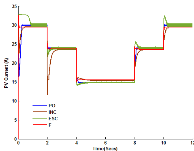
Figure 10 PV output current curves.
