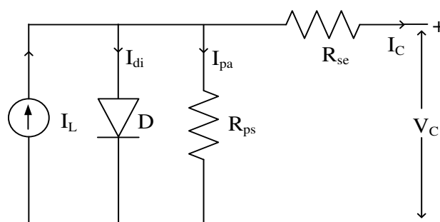
Figure 1 Single diode equivalent model.
