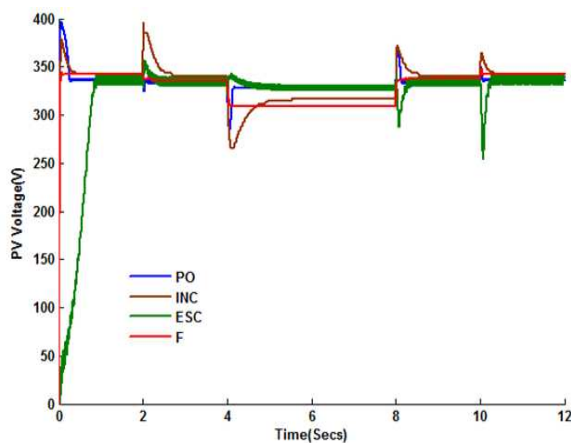
Figure 9 PV output voltage curves.
