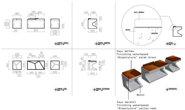
Gambar 6.29. Detail furniture alternatif 1 Sumber: Penulis (2015)
