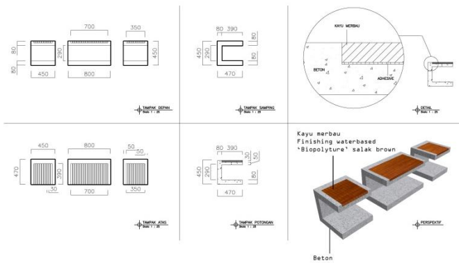
Gambar 6.34. Detail furniture alternatif 2 Sumber: Penulis (2015)
