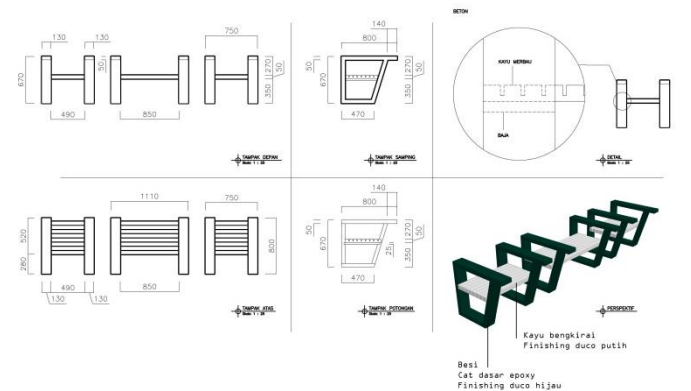
Gambar 6.39. Detail furniture alternatif 3 Sumber: Penulis (2015)
