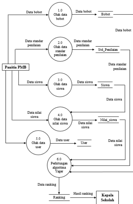
Gambar 3. DFD level 1
