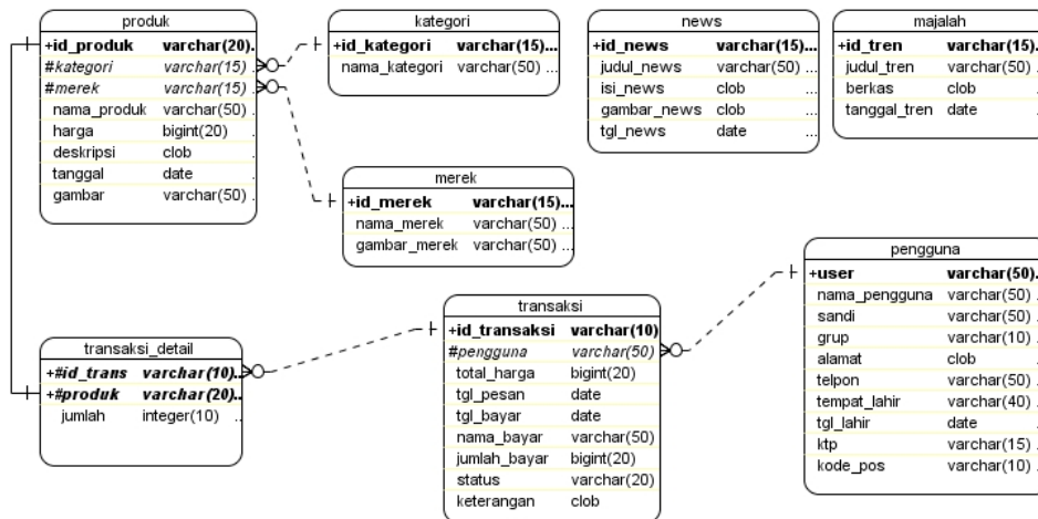
Gambar 3.4 Skema Basis Data
