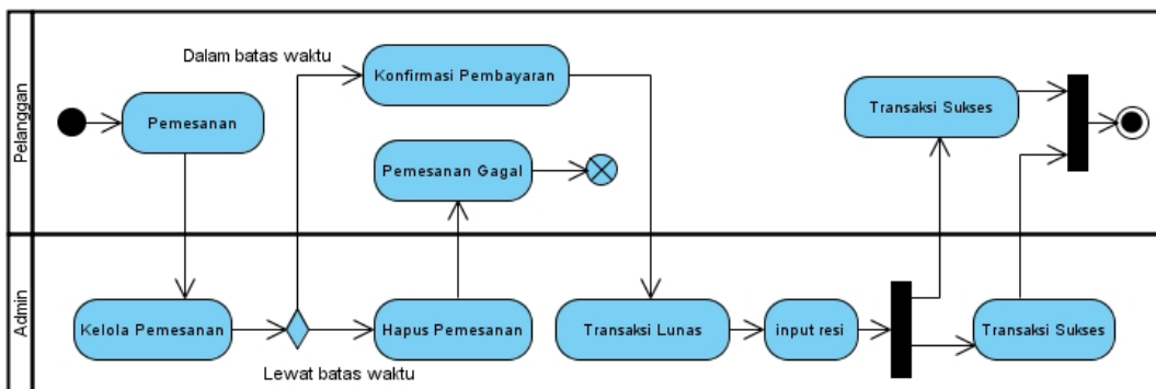
Gambar 3.2 Activity Diagram Global E-Shop
