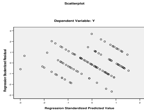
Gambar 2. Scatterplot
