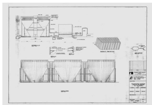
Gambar 5. As built drawing bangunan tangki unit IPA IV
