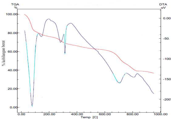
Figure 4. Thermogram of Hydrotalcite
