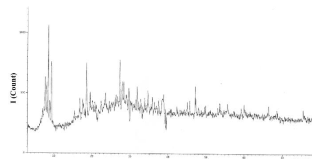
Figure 2. Pattern of polyoxometalate H_4[\alpha-SiW_{12}O_{40}] \cdot nH_2O
