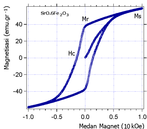
Gambar 3. Kurva histeresis sampel SrO 6 Fe 2 O 3
