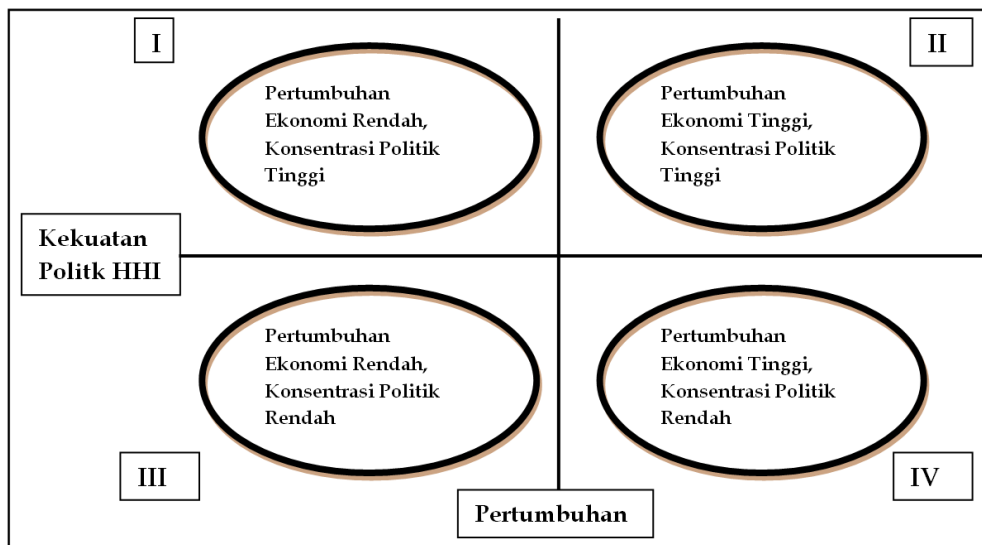
Gambar 1: Diagram Kartesius
