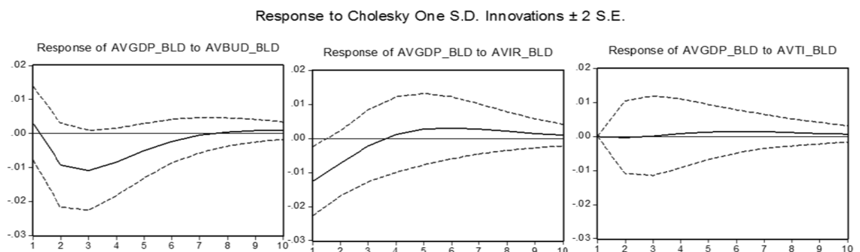
Gambar 7. Impulse Response Belanda
