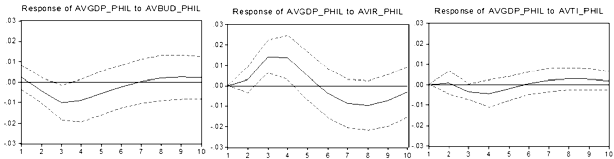
Gambar 4. Impulse Response Filipina
