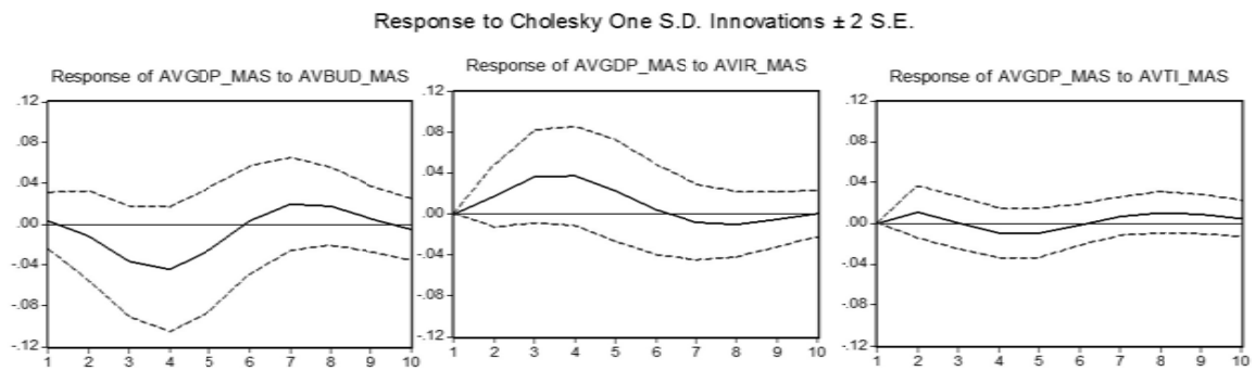
Gambar 3. Impulse Response Malaysia
