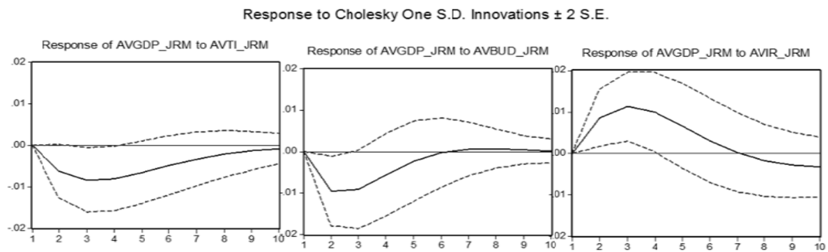
Gambar 6. Impulse Response Jerman
