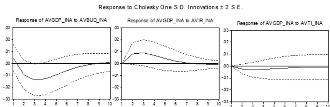
Gambar 2. Impulse Response Indonesia
