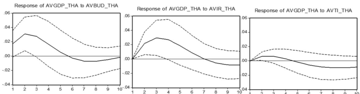
Gambar 5. Impulse Response Thailand
