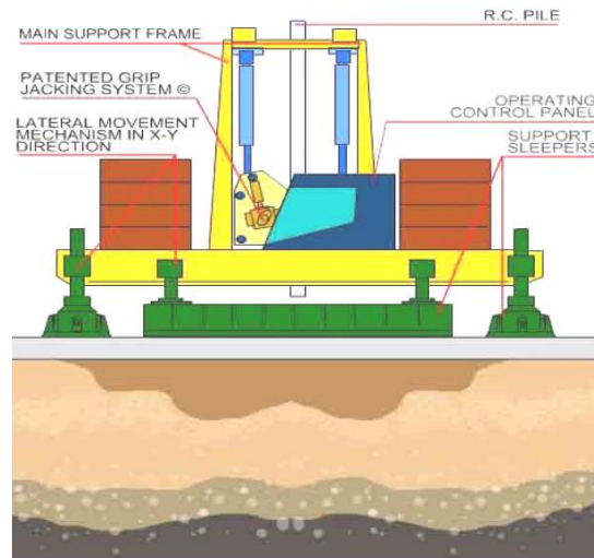
Gambar 1. Hydraulic Static Pile Driver
