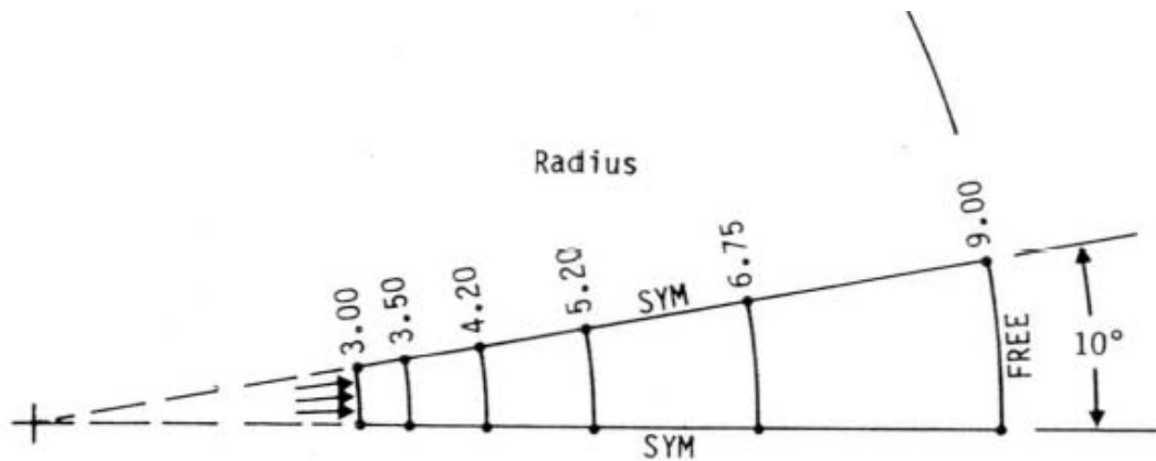
Gambar 5. Thick-Walled Cylinder
