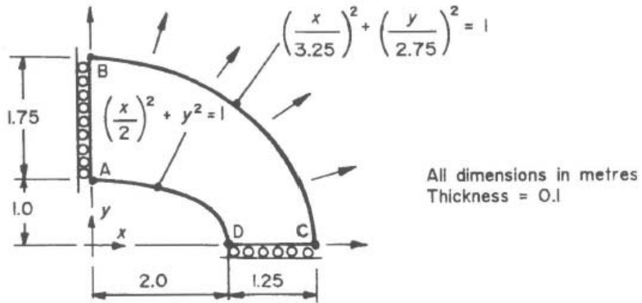
Gambar 4. Elliptic Membrane
