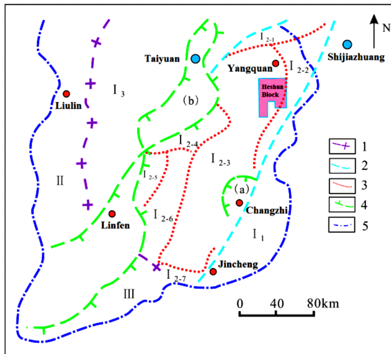
1—primary tectonic boundary; 2—secondary tectonic boundary; 3—third-level tectonic boundary; 4—Cenozoic basin boundary; 5—provincial boundary; I 1 —Lvliang-Taihang fault block; I 2-1 —Taihang block ridge; I 2-2 —Qinshui depression; I 2-3 —Yuxian depression-rim tilting zone; I 2-4 —Niangziguan-Pingtou depression-rim tilting zone; I 2-5 —Zhanshang-Wuxiang-Yangcheng NNE trending fold belt; I 2-6 —Pudong-Laiyuan NEE trending fold-thrust belt; I 2-7 —Taiyue depression-rim tilting zone; I 3 —Guodao-Anze near-NS trending fold belt; II—Xichengshan depression-rim tilting zone; III—Lvliang depression; II—Ordos fault block; III—Henan-Anhui fault block; a—Changzhi new fault depression; b—Taiyuan new fault depression; c—Linfen new fault depression
