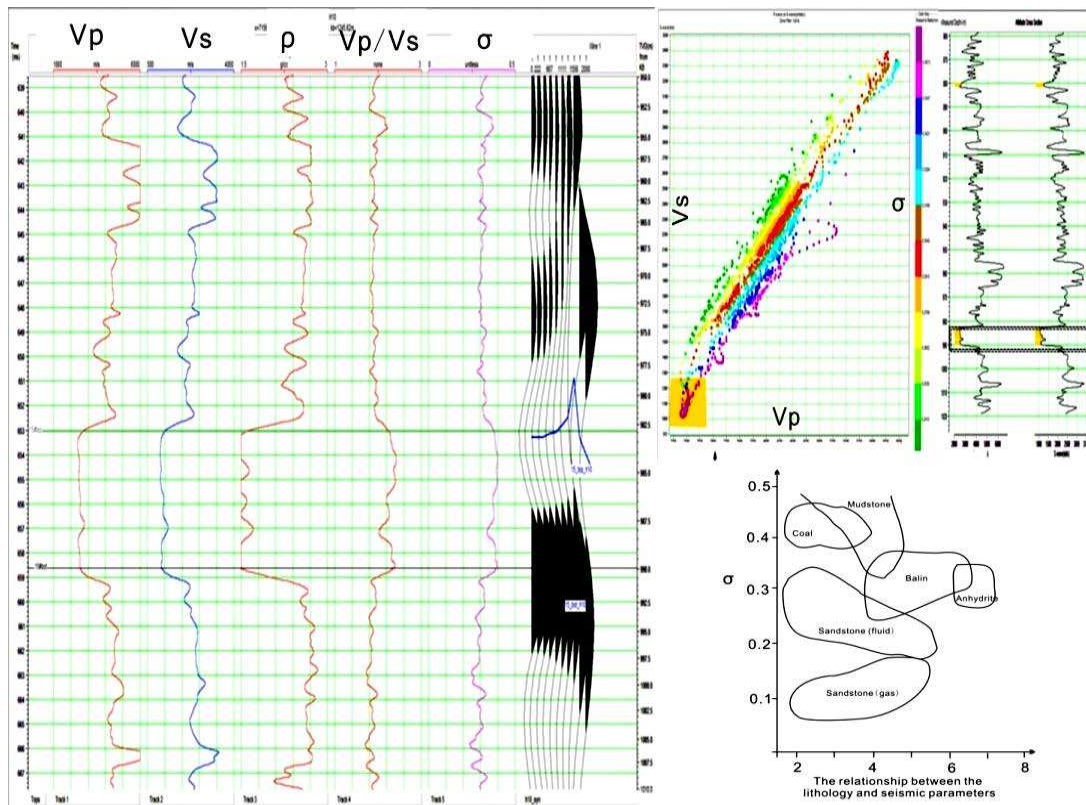
Figure 7 Well logging data analysis map for H10.
