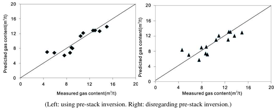
Figure 10 Correlation coefficient graphs the measured gas content vs. predicted gas content at the drilling wells.
