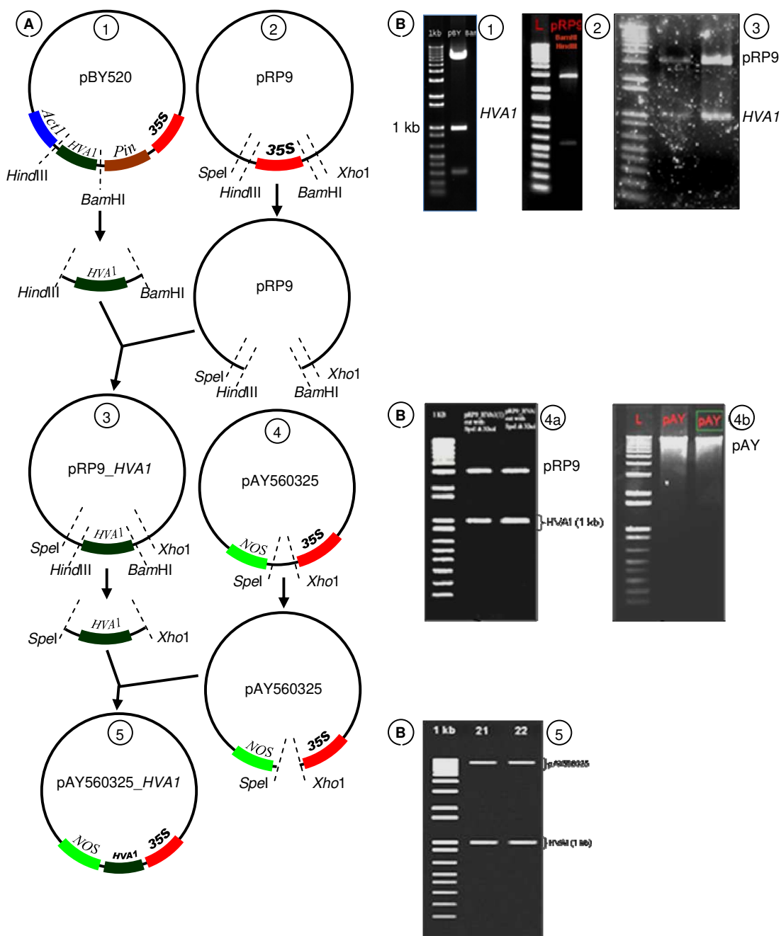
Figure 1. Construction strategy of HVA1 binary expression vector. A = Schematic construction of HVA1 binary expression vector: (1) Hva1 gene was cut off from plasmid pBY520 using Hind III- Bam HI restriction enzymes; (2) Subcloning Hva1 gene into plasmid pRP9, which was digested with the same enzymes to generate pRP9_ HVA1 ; (3) HVA1 gene was cut out of the pRP9_ HVA1 using Spe I- Xho I enzymes and inserted into 35S-Nos promoter-terminator in pAY560325; (4) pAY560325 was cut with the same enzymes to generate pAY560325_ HVA1 (5). B = gel electrophoresis for extractions of HVA1 binary expression vector: (1) HVA1 gene was cut out from plasmid pBY520 using Hind III- Bam HI. (2 + 3) The HVA1 gene was subcloned into pRP9 plasmid, which was digested with the same enzymes, to generate pRP9_ HVA1 ; (4a) HVA1 was cut out from the pRP9_ HVA1 using Spe I- Xho I, and (4b) HVA1 was inserted into 35S-Nos promoter-terminator in pAY560325, which was cut with the same enzymes to generate 5 pAY560326_ HVA1 .
