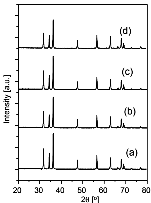
Figure 7 Powder XRD patterns of samples, showing the effect of PEG content on the crystallinity: (a) no PEG, (b) PEG 2 g, (c) PEG 4 g, and (d) PEG 8 g. Various polymer weights were added in 10 mL solution of zinc acetate 0.6 M. The precursors were heated at 800°C for 30 min.
