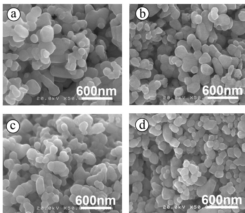
Figure 6 SEM pictures of samples, showing the effect of PEG content on the morphology: (a) no PEG, (b) PEG 2 g, (c) PEG 4 g, and (d) PEG 8 g. Various polymer weights were added in 10 mL solution of zinc acetate 0.6 M. The precursors were heated at 800°C for 30 min.
