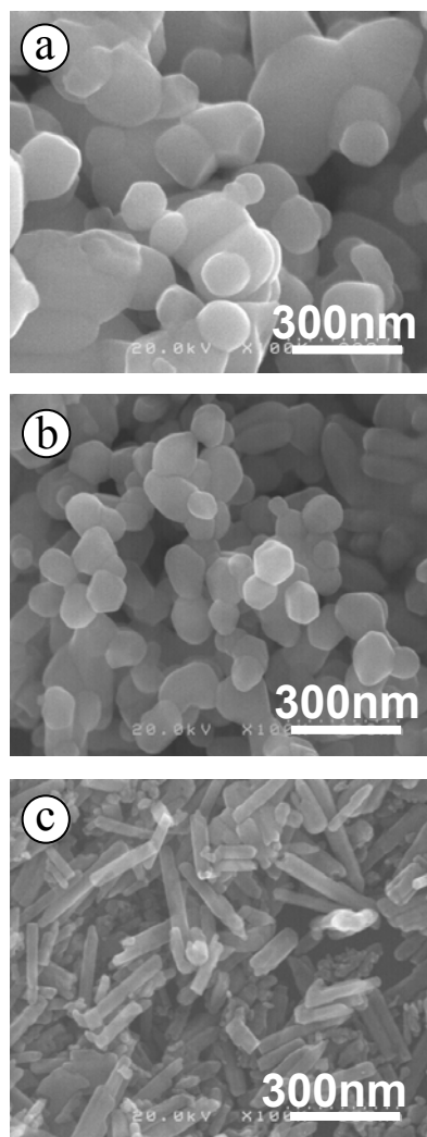
Figure 8 SEM pictures of samples, showing the effect of heating temperature on the morphology: (a) 800°C, (b) 600°C, and (c) 400°C. The precursors are 10 mL solutions of zinc acetate 0.6 M, heated for 30 min.
