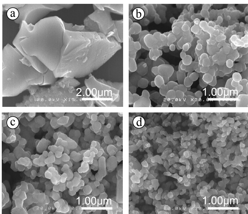
Figure 1 SEM pictures of samples, showing the effect of PEG content on the morphology: (a) no PEG, (b) PEG 4 g, (c) PEG 8 g, and (d) PEG 12 g. Various polymer weights were added in 10 mL solution of zinc nitrate 0.6 M. The precursors were heated at 800°C for 30 min.
