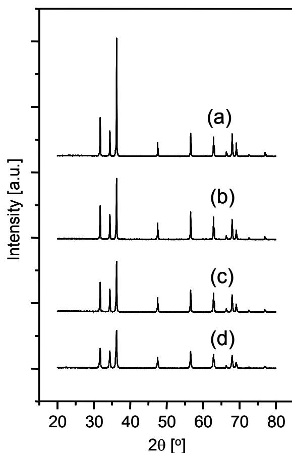
Figure 2 Powder XRD patterns of samples, showing the effect of PEG content on the crystallinity: (a) no PEG, (b) PEG 4 g, (c) PEG 8 g, and (d) PEG 12 g. Various polymer weights were added in 10 mL solution of zinc nitrate 0.6 M. The precursors were heated at 800°C for 30 min.
