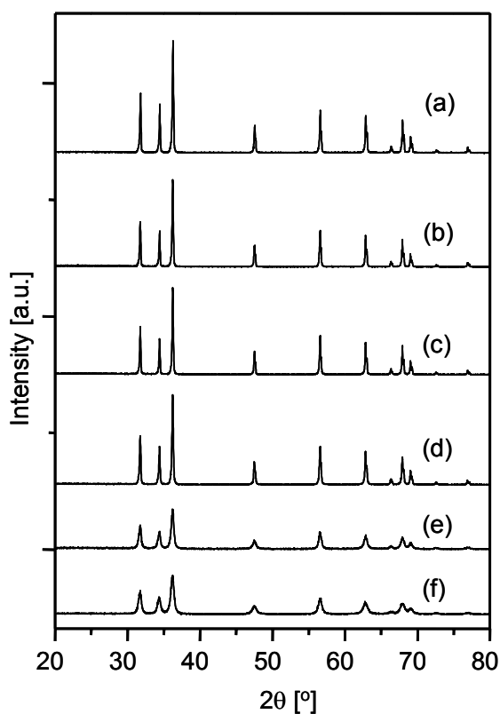
Figure 4 Powder XRD patterns of samples, showing the effect of heating temperature on the crystallinity: (a) 1000°C, (b) 900°C, (c) 800°C, (d) 700°C, (e) 600°C, and (f) 500°C. PEG 8 g was added in 10 mL solution of zinc nitrate 0.6 M and the precursors were heated for 30 min.
