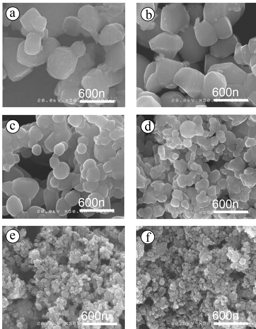
Figure 3 SEM pictures of samples, showing the effect of heating temperature on the morphology: (a) 1000°C, (b) 900°C, (c) 800°C, (d) 700°C, (e) 600°C, and (f) 500°C. PEG 8 g was added in 10 mL solution of zinc nitrate 0.6 M and the precursors were heated for 30 min.
