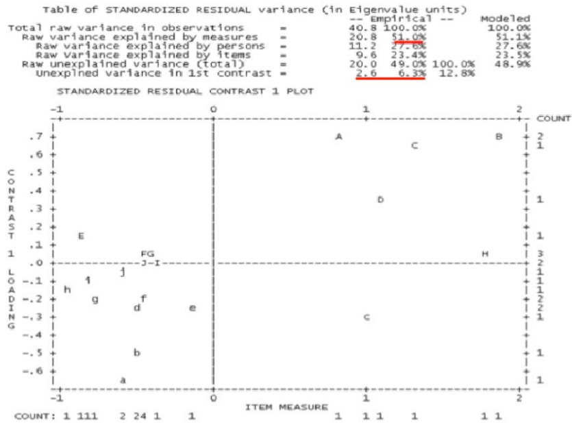
Figure 3. Item Dimensionality
