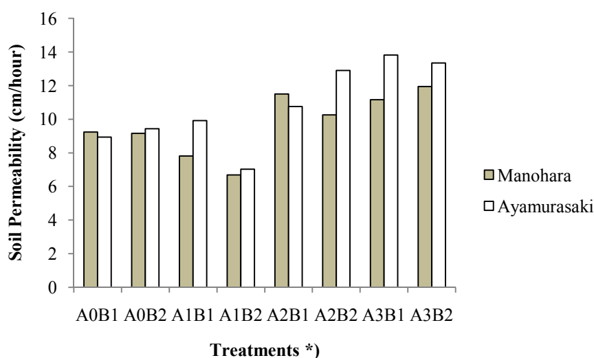
Figure 1. Effects of application of volcanic ash and compost on permeability of a sandy soil. *) A0 = 100% soil, A1 = 10% volcanic ash + 90% soil, A2 = 20% volcanic ash + 70% soil, A3 = 30% volcanic ash + 70% soil, B1 = 2.5 t compost/ha, B2 = 5 t compost/ha
