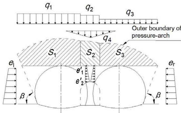
Figure 4 Schematic of the pressure-arch and the simplified loads.
