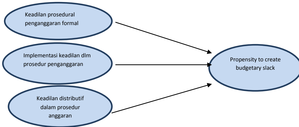
Gambar 1 Model Penelitian
