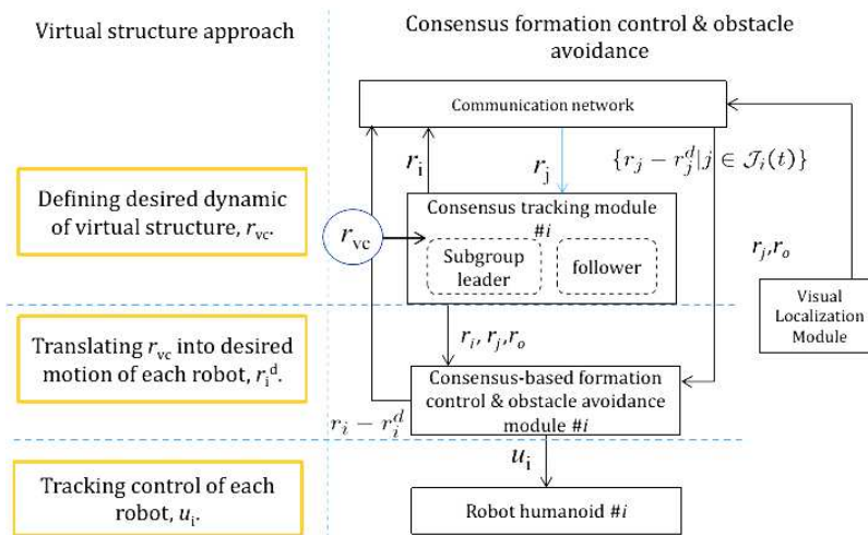
Figure 8. The elaboration of VS approach into distributed architecture for obstacle/collision avoidance and formation control [3]
