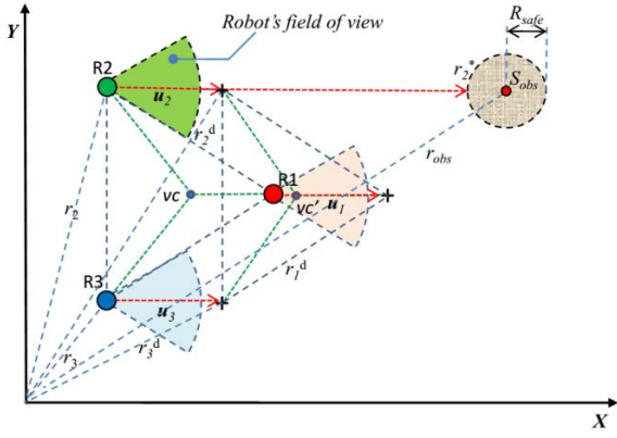
Figure 7. Illustration of obstacle/collision avoidance and formation control
