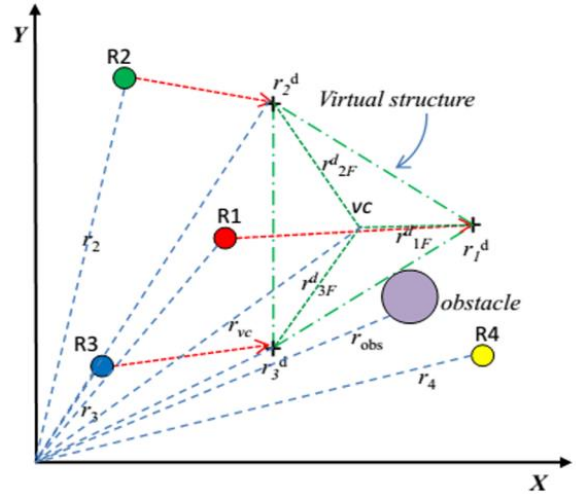
Figure 1. A formation composed of three robots with a known virtual center & an obstacle
