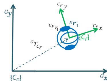
Figure 2. Frame coordinate transformation from global into robot's frame coordinate
